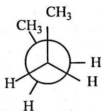
Eclipsed
