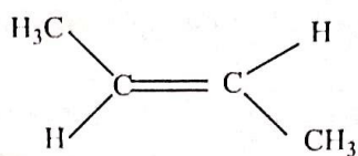
Trans isomer
