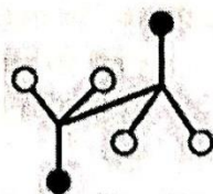
anti conformation
