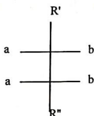
erythro form
