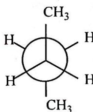
Anti
