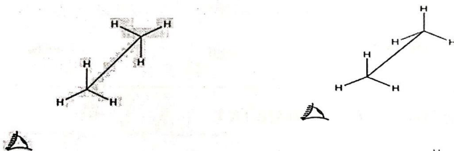
Anti conformation
