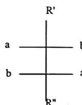
threo form
