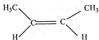
Cis isomer
