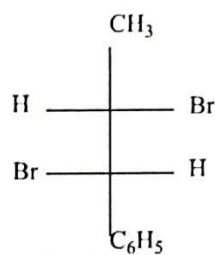
threo form
