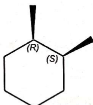
Cis isomer
