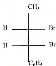
erythro form
