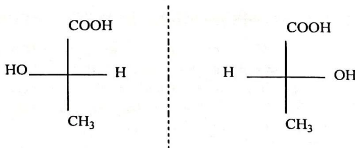
Two isomers of Lactic acid
