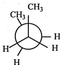
Eclipsed
