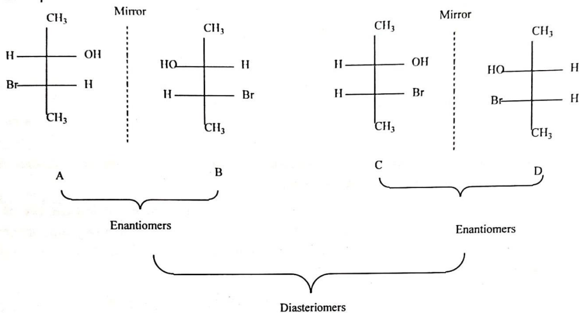
Four isomers of 3-Bromo-2-butanol
