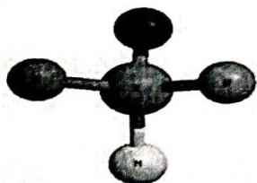
“Ball and stick” model of 3-D structure of methane
