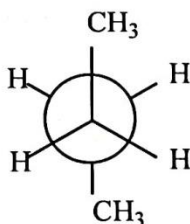
Anti
