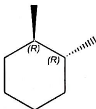
Trans isomer
